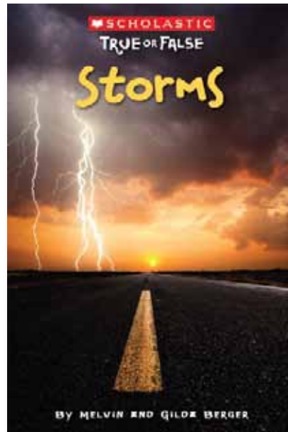
#7: STORMS
